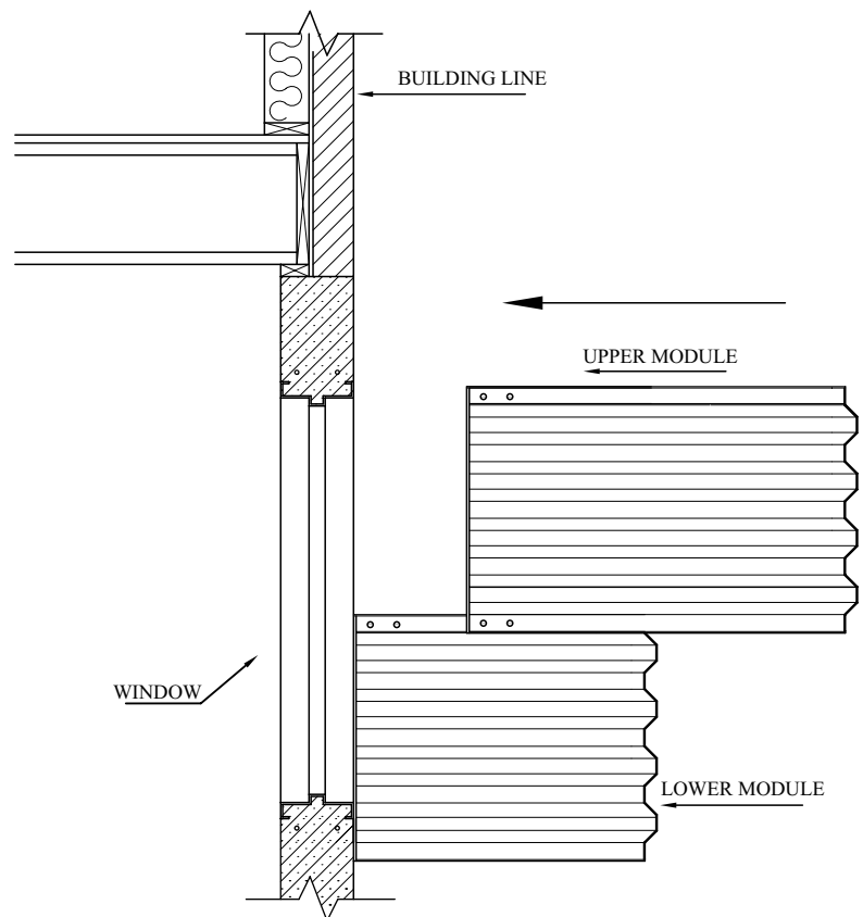
Figure 1. Tier 2 Installation
