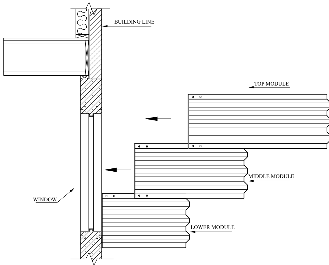
Figure 2. Tier 3 Installation
